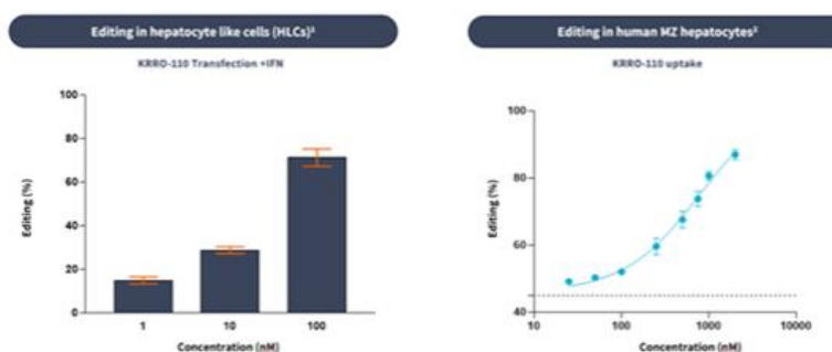
Figure 14. KRRO-110 demonstrated >50% editing in in vitro systems with the Z genotype
