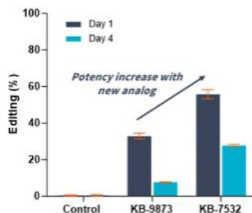
Figure 5. We have a demonstrated ability to improve editing in target coding regions
