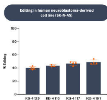
Figure 28. Editing of TDP-43 mRNA using our product candidates (100 nM)
