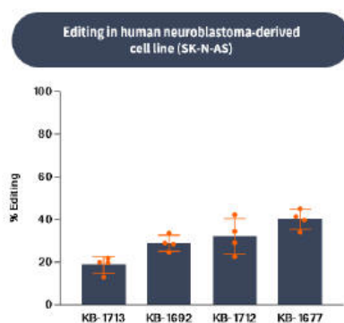
Figure 29. Editing of Nav1.7 using our product candidates (100nM)
