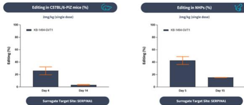
Figure 21. Editing of SERPINA1 coding region in NHPs and C57BL/6-PtZ model showed correlation
