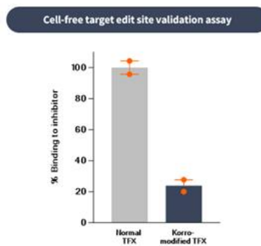
Figure 23. Changing a single amino acid disrupts binding of a transcription factor to its inhibitor
