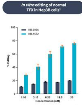
Figure 24. Our product candidate edits transcription factor RNA at the validated target site in a dose-responsive manner
