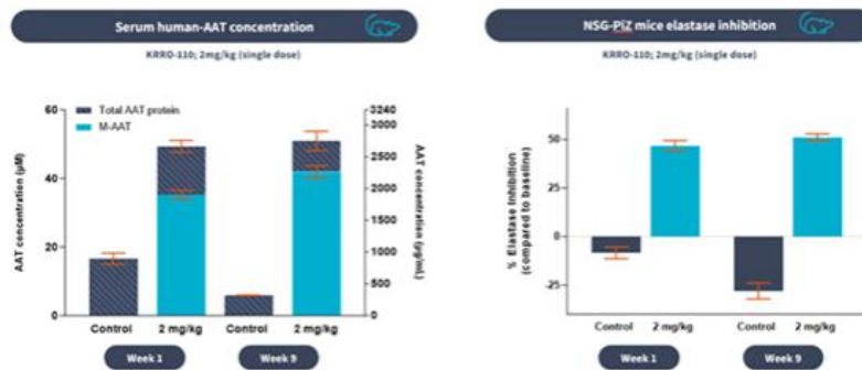
Figure 17. Secretion of functional AAT (approximately 50µM) as early as 7 days post-single dose
