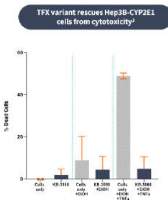
Figure 26. RNA editing demonstrates increased viability of liver cells in an in vitro model of sAH
